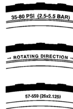
Tire markings
